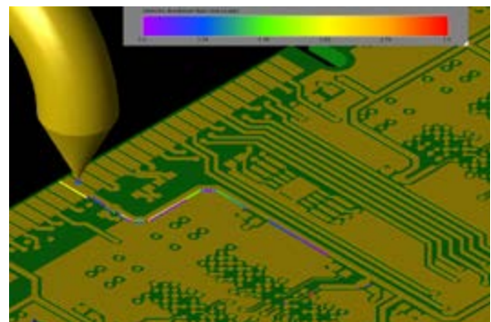
Cell edges which exceeded their dielectric strength during a simulation can be examined with the Dielectric Breakdown Sensor and Dielectric Breakdown Ratio result type.
